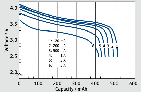
Discharge Curves at RT
