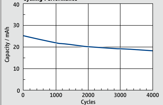
Cycling Performance
