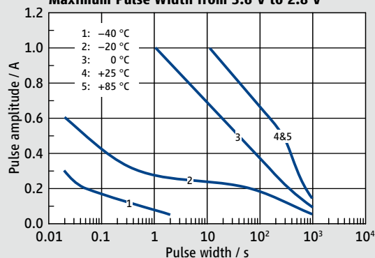
Maximum Pulse Width from 3.6 V to 2.8 V
