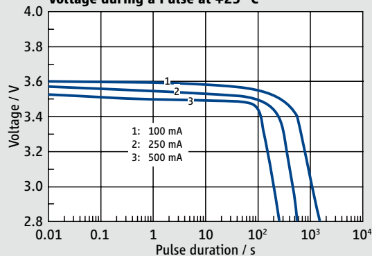
Voltage during a Pulse at +25 °C
