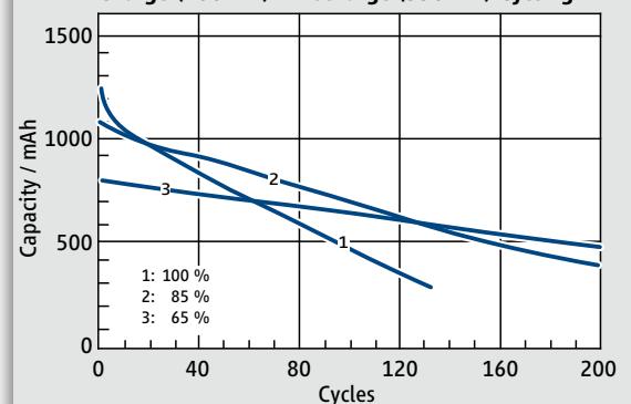
Charge (100 mA) / Discharge (350 mA) Cycling
