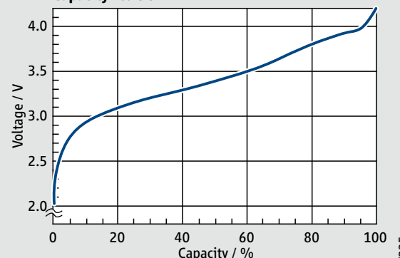
Capacity vs. OCV
