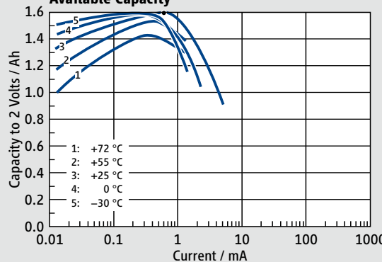
Available Capacity
