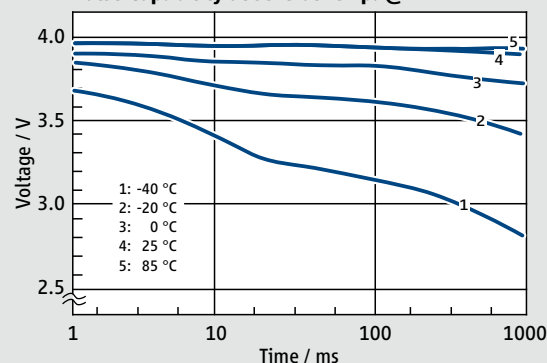
Pulse Capability at several Temp. @ 2 A
