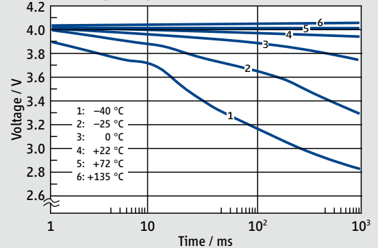
Pulse Capability at 1 A
