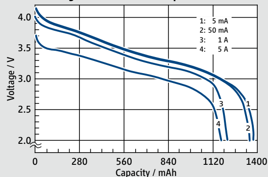
Discharge Curves at Room Temperature
