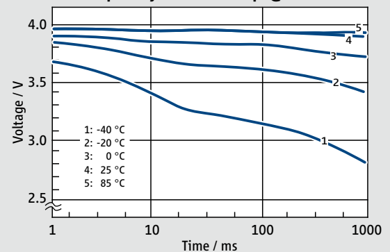
Pulse Capability at several Temp. @ 2 A
