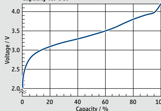
Capacity vs. OCV
