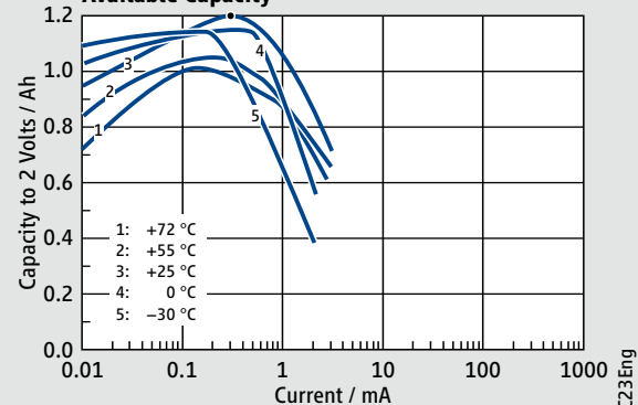
Available Capacity
