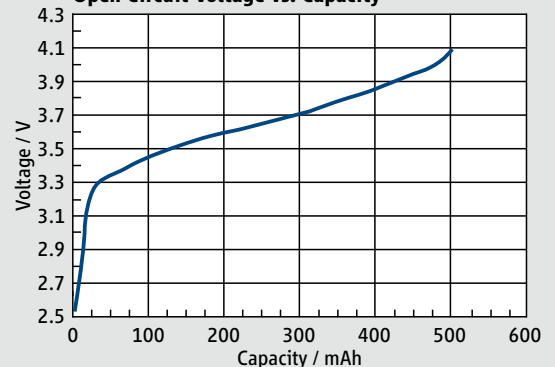
Open Circuit Voltage vs. Capacity
