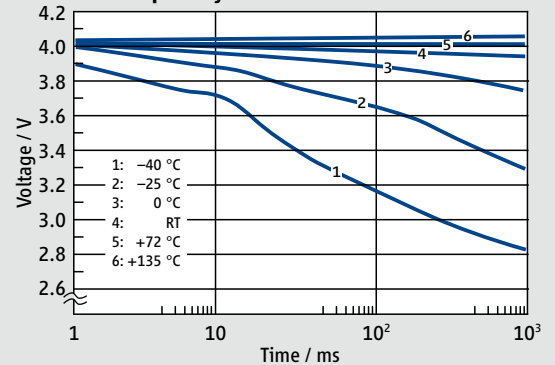
Pulse Capability at 1 A
