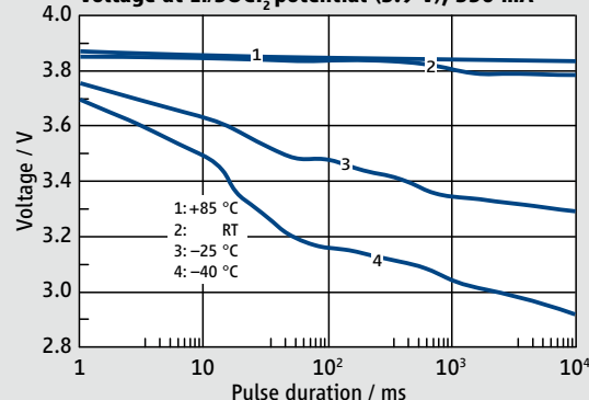
Voltage at Li/SOCl 2 potential (3.9 V), 350 mA
