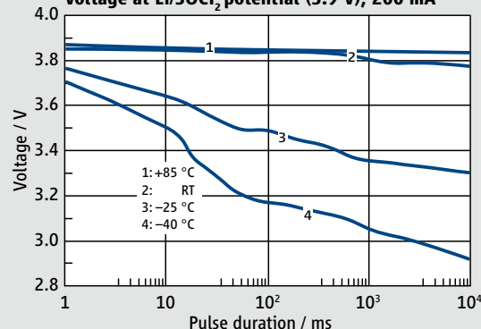
Voltage at Li/SOCl 2 potential (3.9 V), 200 mA
