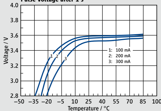
Pulse Voltage after 1 s
