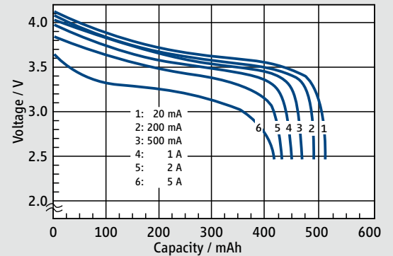
Discharge Curves at Room Temperature
