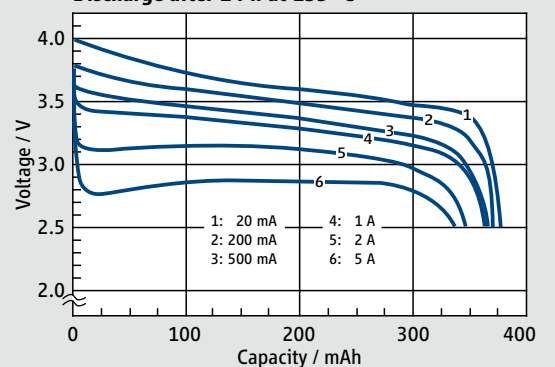
Discharge after 24 h at 135 °C
