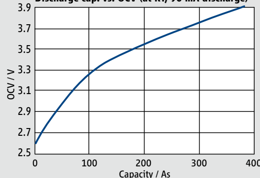
Discharge cap. vs. OCV (at RT, 90 mA discharge)
