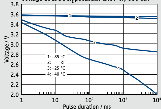
Voltage at Li/SOCl 2 potential (3.67 V), 600 mA
